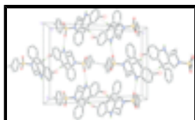
Fig. 3. Part of the three-dimensional network in the title compound. Dashed and dotted lines indicate N—H...O and C—H... \pi interactions, respectively. The \pi - \pi interaction is shown by a dashed open line. For the sake of clarity, H atoms not involved in the interactions have been omitted.
